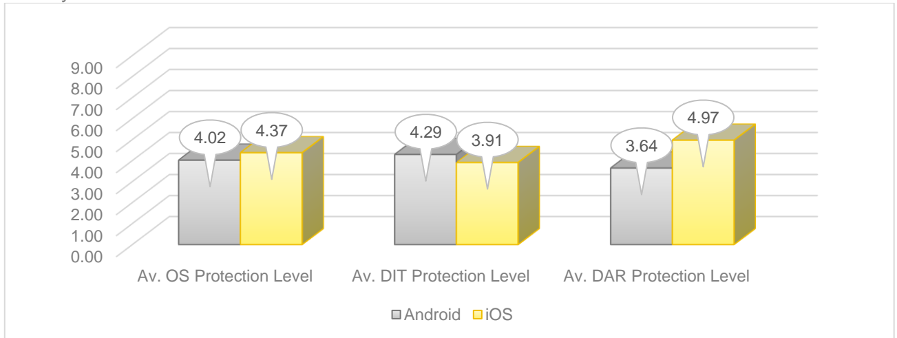
FIGURE 1. AVERAGE PROTECTION LEVELS OVER 250 APPLICATIONS. ENVIRONMENTAL LEVEL
