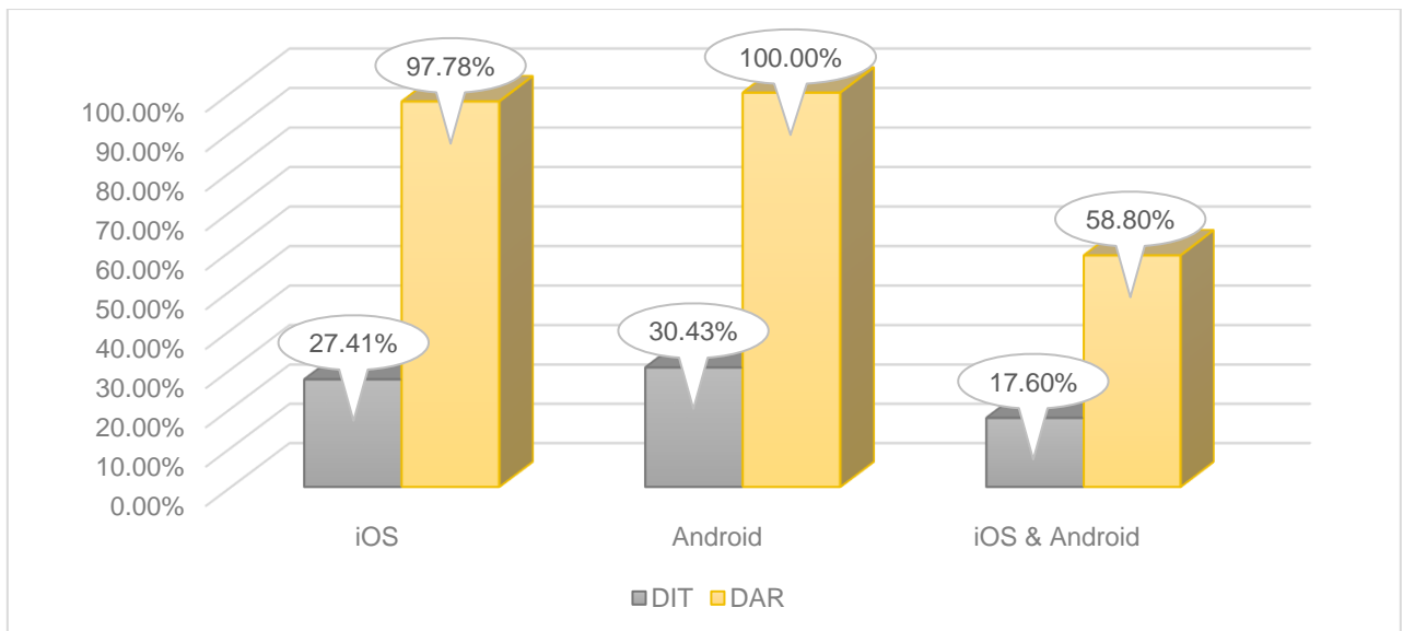
FIGURE 4. QUANTITY OF APPLICATION WITHOUT DATA ENCRYPTION
