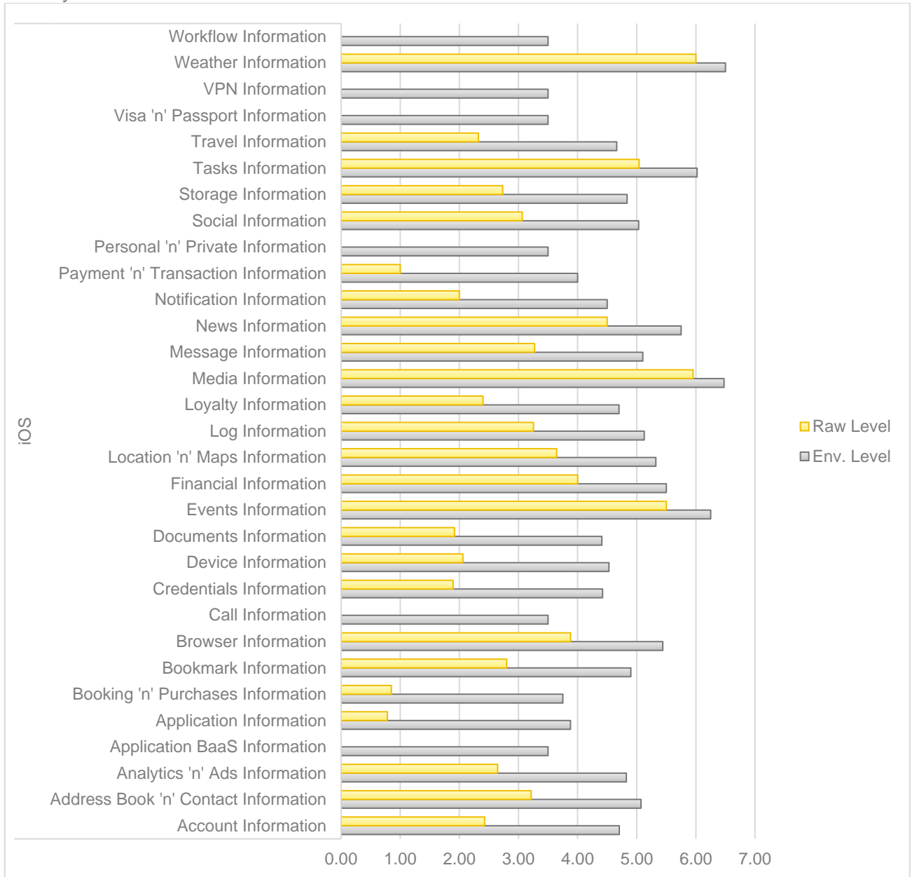
FIGURE 11. DATA GROUPS' OVERALL PROTECTION. IOS. DATA-AT-REST
