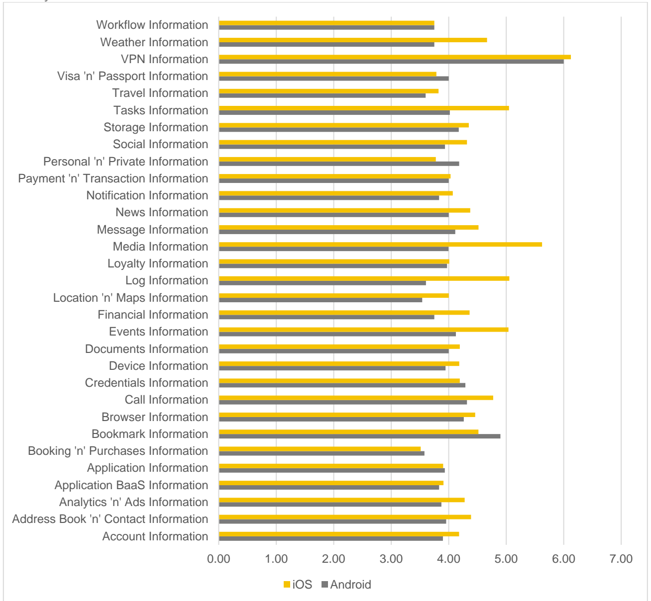
FIGURE 9. DATA GROUPS' AVERAGE PROTECTION LEVEL. IOS VS. ANDROID. COMPARISON CHART
