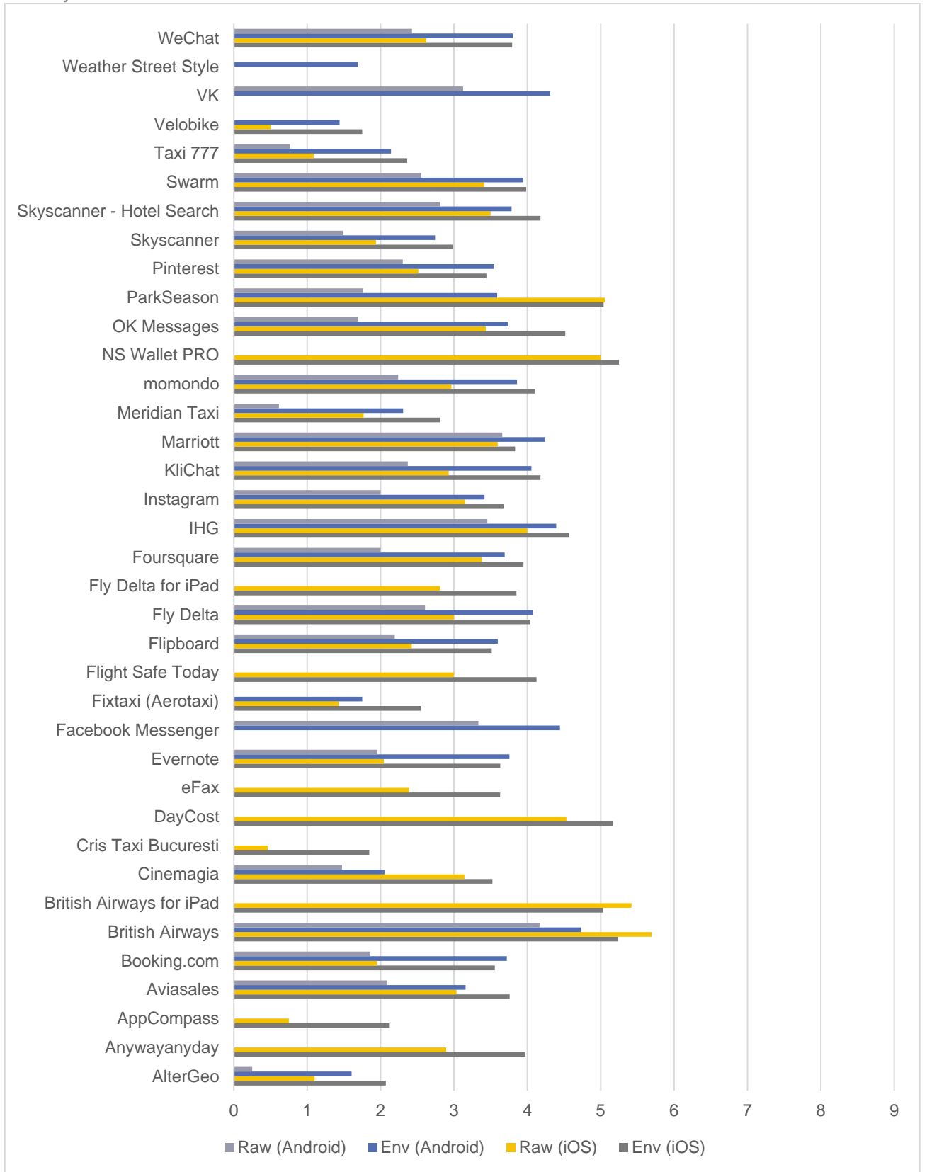
FIGURE 3. APPLICATIONS WITH WORST PROTECTED ITEMS (NON-PROTECTED ITEMS)
