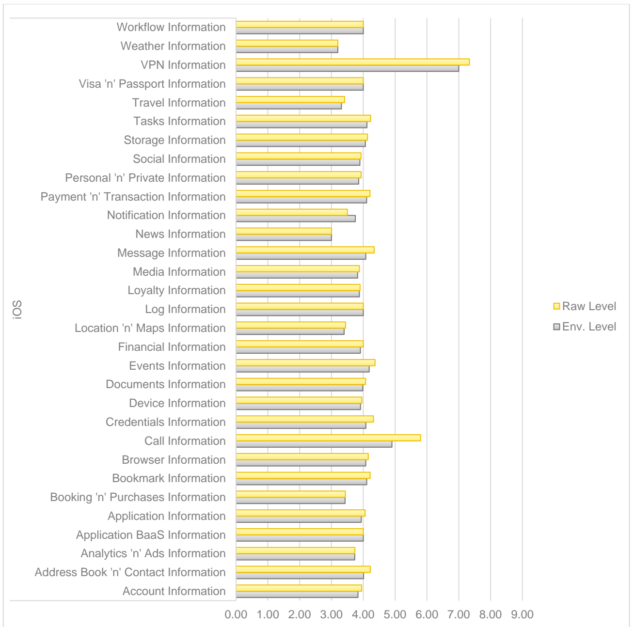
FIGURE 10. DATA GROUPS' OVERALL PROTECTION. IOS. DATA-IN-TRANSIT
