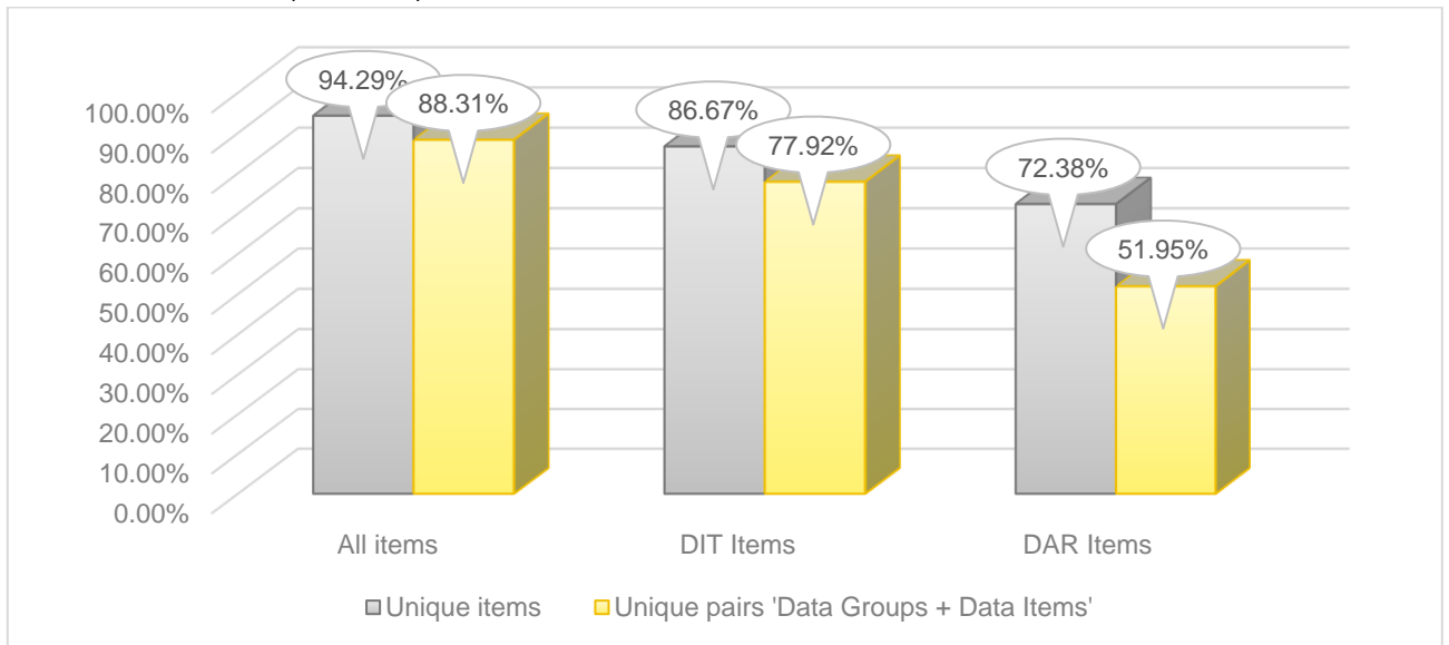
FIGURE 17. THE QUANTITY OF BADLY PROTECTED ITEMS. IOS APPLICATIONS
