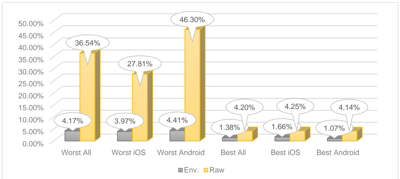
FIGURE 6. THE QUANTITY OF PROTECTED DATA ITEMS VS. OS IMPACT. COMPARISON CHART
