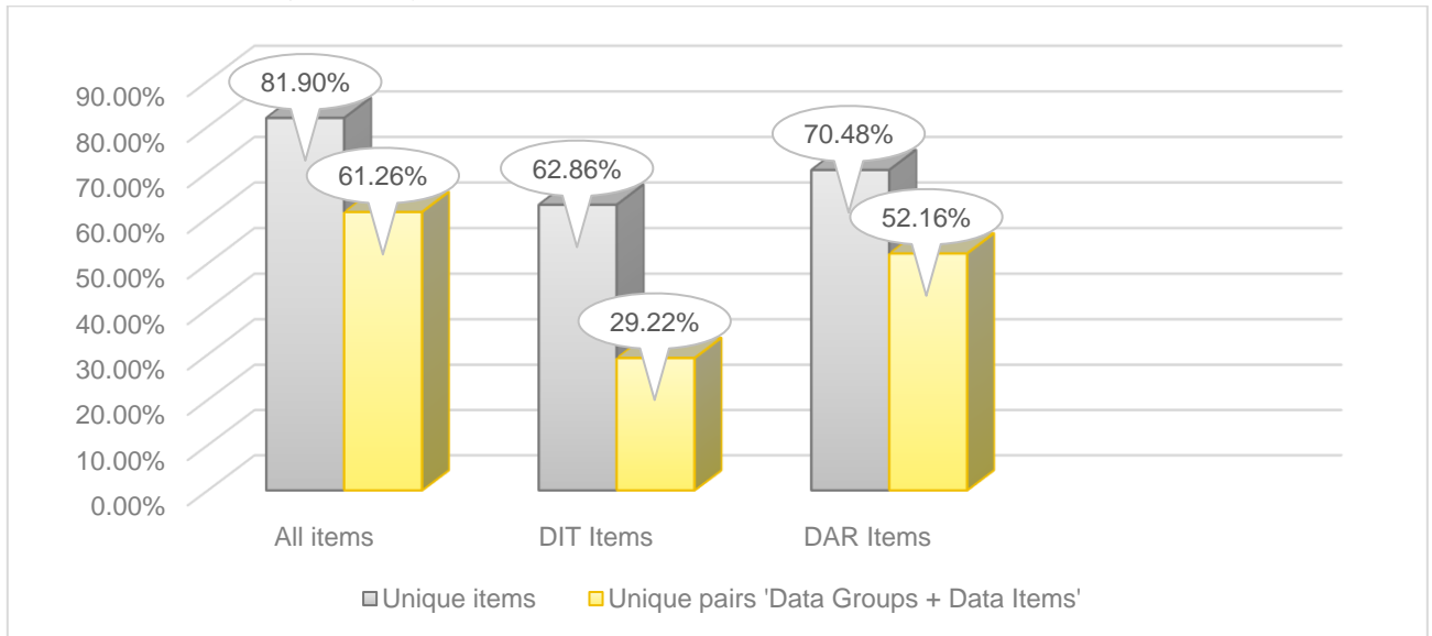
FIGURE 19. THE QUANTITY OF GOOD PROTECTED ITEMS. IOS APPLICATIONS
