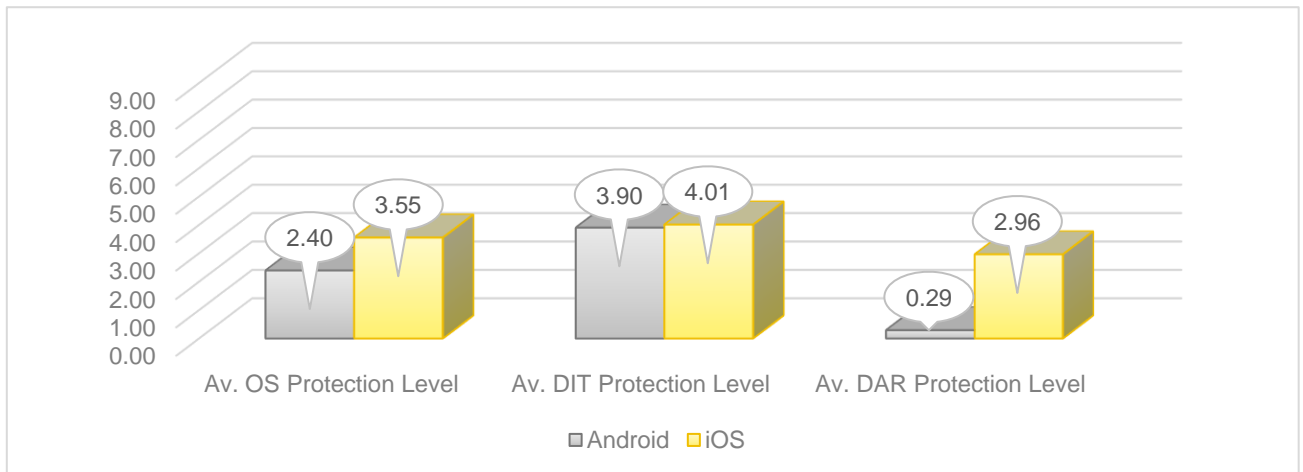
FIGURE 2. AVERAGE PROTECTION LEVELS OVER 250 APPLICATIONS. RAW LEVEL
