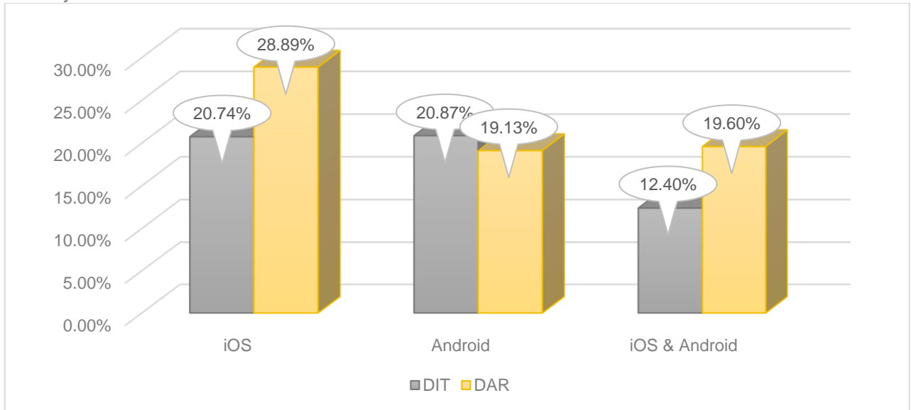
FIGURE 5. QUANTITY OF APPLICATION WITH DATA ENCRYPTION
