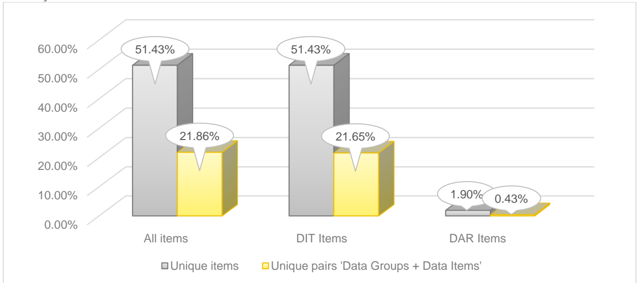
FIGURE 20. THE QUANTITY OF GOOD PROTECTED ITEMS. ANDROID APPLICATIONS
