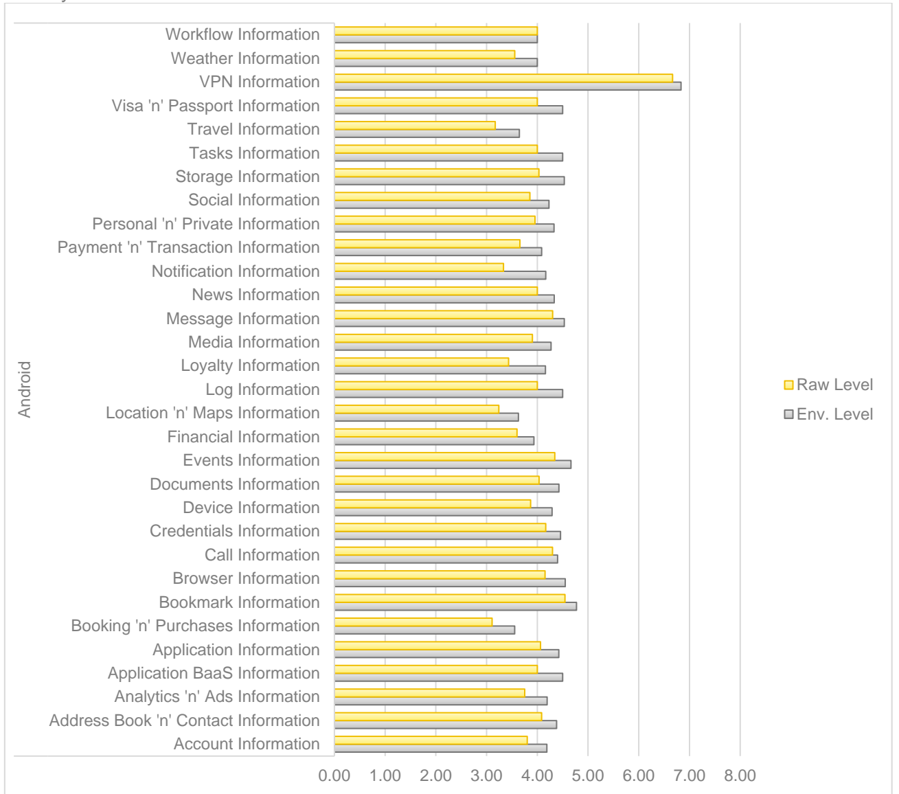
FIGURE 12. DATA GROUPS' OVERALL PROTECTION. ANDROID. DATA-IN-TRANSIT
